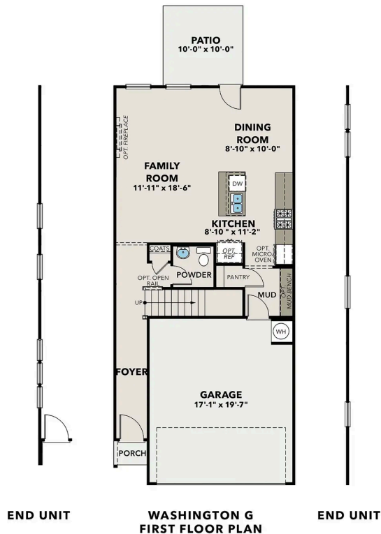
THE WASHINGTON FIRST FLOOR
