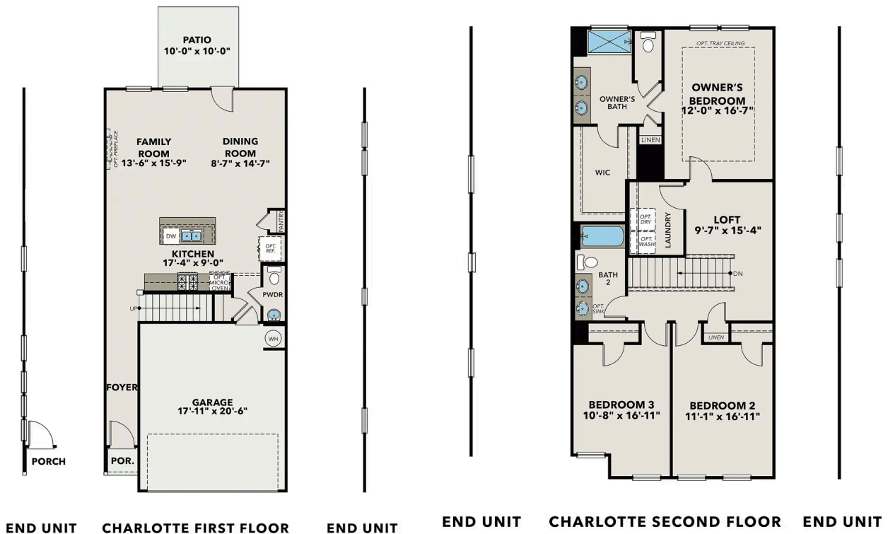
THE CHARLOTTE FIRST FLOOR
